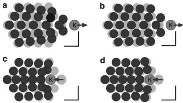
FIGURE 9 ULs can prevent stereocilia from fusing. For this simulation, an ideally symmetric hair bundle was used to avoid possible artifacts of irregular stereocilia spacing. Each plot shows the top view of a deformed hair bundle. Undeformed configurations are shown as background shadows. Top and bottom plots show hair bundles subjected to 400 pN at the tip of kinocilium in the excitatory and 200 pN in the inhibitory directions, respectively. Left plots ( a and c ) show the results when allowing contact between stereocilia. Without something to separate them, some stereocilia may fuse together. In the plots at right ( b and d ), the ULs are used as a separator or a contact element. The ULs prevented the stereocilia from contacting each other directly.
