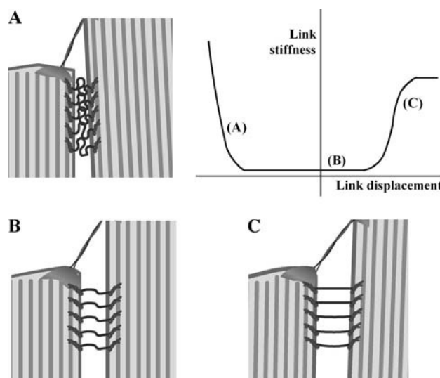
FIGURE 8 Stiffness characteristics of ULs. This study suggests that the stiffness of ULs is nonlinear. In the resting state (b), the UL has little stiffness. As it stretches during an excitatory deflection (c), it uncoils and becomes stiffer. During an inhibitory deflection (a), it behaves like a contact element that prevents the neighboring stereocilia from fusing. This study focused on the initial or resting stiffness when the tip displacement is very small (less than a few nanometers). Within this small displacement range, the ULs are coiled (b) and their stiffness is minimal.
